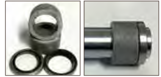
The seals now have a heavy duty steel outer edge with a Teflon lipped seal.
